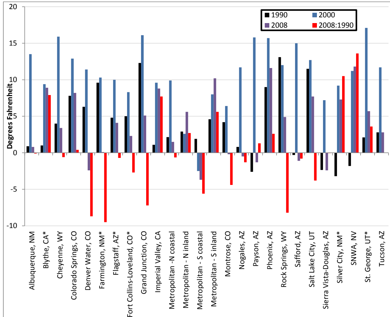
Figure B-2. Combined May-September Deviation From Average Monthly Temperature, for Water Agency Areas.
