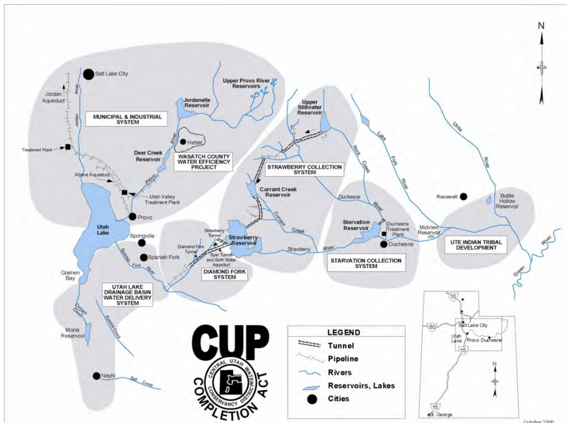
Figure 5. The Bonneville Unit System.
