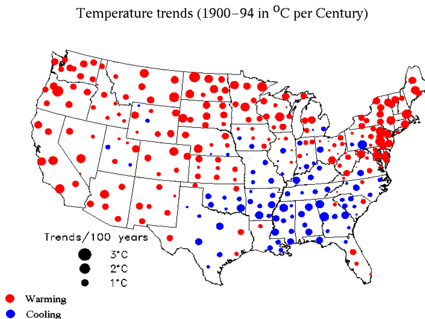
Figure 7: Temperature Trends in the Continental United States (1900 to 1994)
