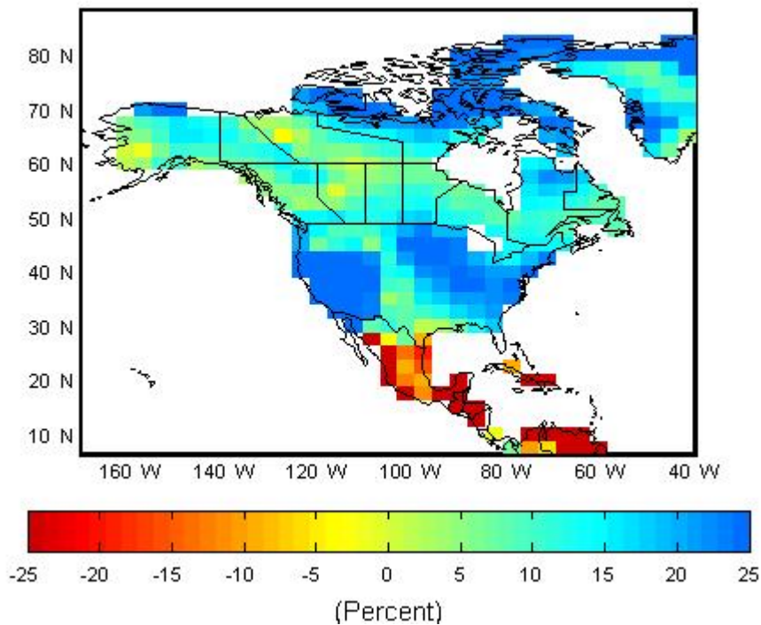
Figure 2b: Hadley2 model precipitation changes for 2080, showing projected increases in precipitation in the western United States. http://www.cics.uvic.ca/scenarios/index.cgi
