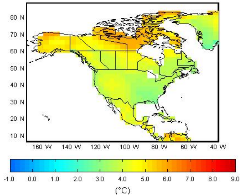
Figure 2a: Hadley2 model temperature changes for 2080 showing increases of 2 to 5 degrees C for the western United States. http://www.cics.uvic.ca/scenarios/index.cgi
