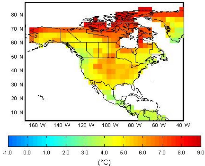
Figure 2c: Canadian model 1 showing temperature changes across North America for 2080, including 3 to 7 degrees C temperature increases in the western United States.
