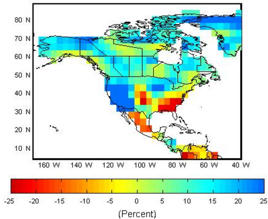
Figure 2d: Canadian climate model precipitation changes for 2080 showing substantial precipitation increases in the western United States. http://www.cics.uvic.ca/scenarios/index.cgi
